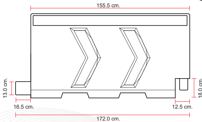
VISTA FRONTAL
