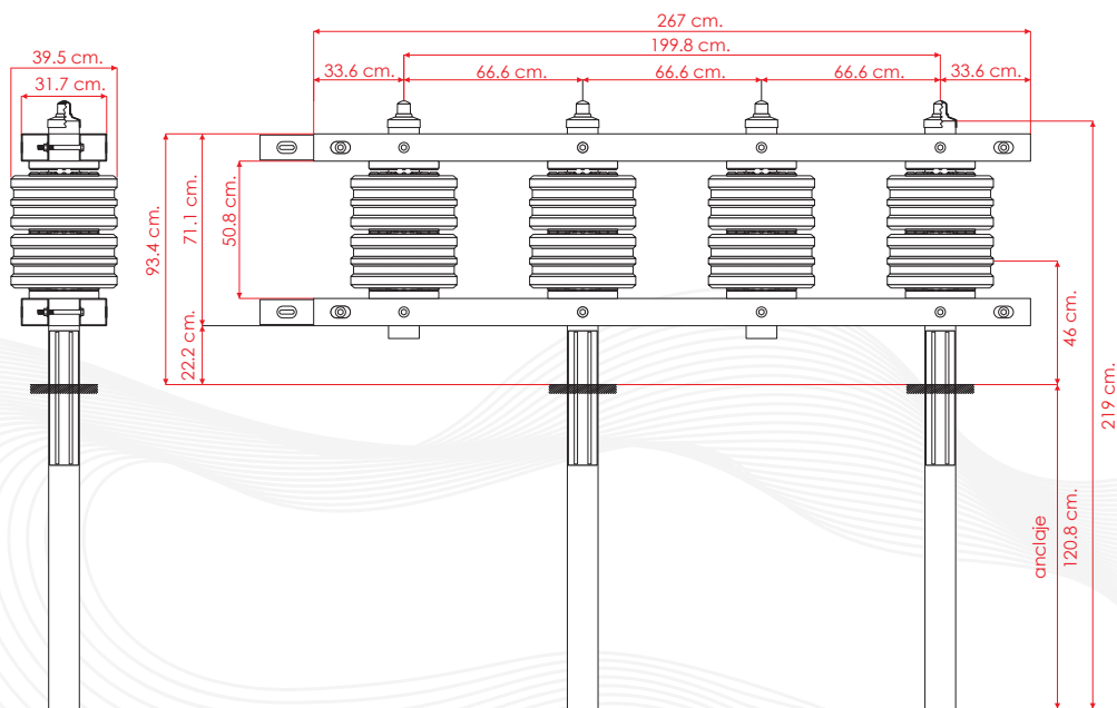
VISTA FRONTAL
